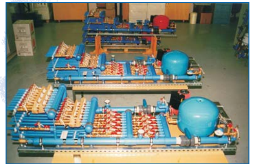
Fabrication of storey stations and distributors according to plan
